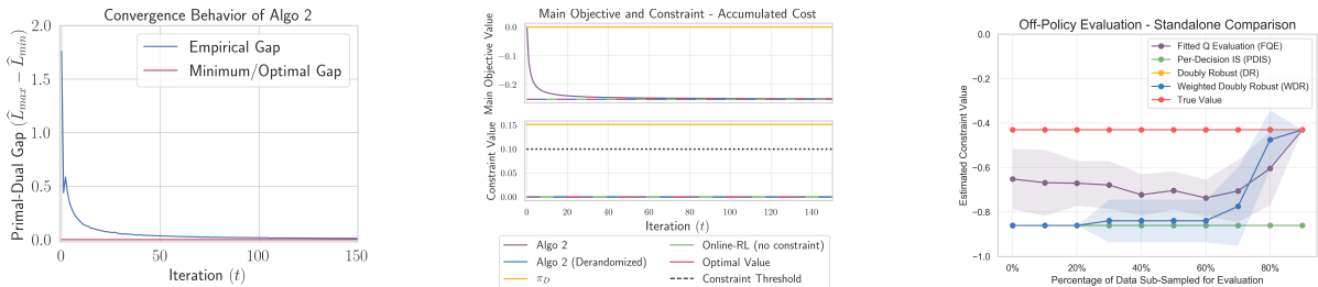
Figure 1. FrozenLake Results. (Left) Empirical duality gap of algorithm 2 vs. optimal gap. (Middle) Comparison of returned policy and others w.r.t. (top) main objective value and (bottom) safety constraint value. (Right) FQE vs. other OPE methods on a standalone basis.
