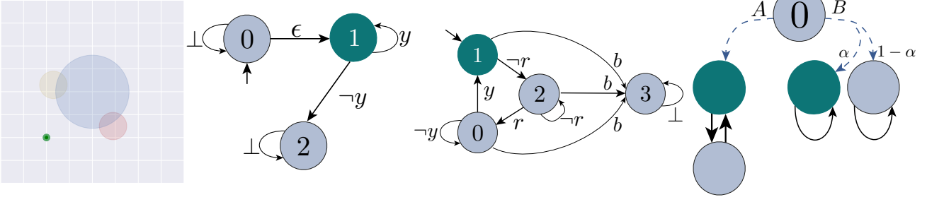
Figure 1. Examples. First: Illustration of the Flatworld environment. The agent is a green dot and there are 3 zones: yellow, blue and red. Second: LDBA \mathcal{B} for “ FGy ”. \mathcal{S}^{\mathcal{B}^*} = \{1\} , denoted by green circle. The initial state is b_{-1} = 0 . Third: LDBA \mathcal{B} for “ GF(y \ \& \ XFr) \ \& \ G\neg b ”. \mathcal{S}^{\mathcal{B}^*} = \{1\} , denoted by green circle. The initial state is b_{-1} = 1 . Fourth: For this example, an agent starting in state 0 and solving \arg \max_{\pi \in \Pi} \mathbb{E}_{\tau \sim T_{\pi}^P} [\sum_{i=0}^{\infty} \gamma^i \mathbf{1}_{\{b_i \in \mathcal{S}^{\mathcal{B}^*}\}}] where \mathcal{S}^{\mathcal{B}^*} is illustrated as the green circles would choose to take action B with probability 1 if \alpha \in (1/2, 1) for any \gamma \in [0, 1] . Such a policy has \mathbb{P}[\pi \models \varphi] = \alpha < 1 . However the probability optimal policy deterministically takes action A , with \mathbb{P}[\pi^* \models \varphi] = 1 . This illustrates catastrophic myopic behavior.
